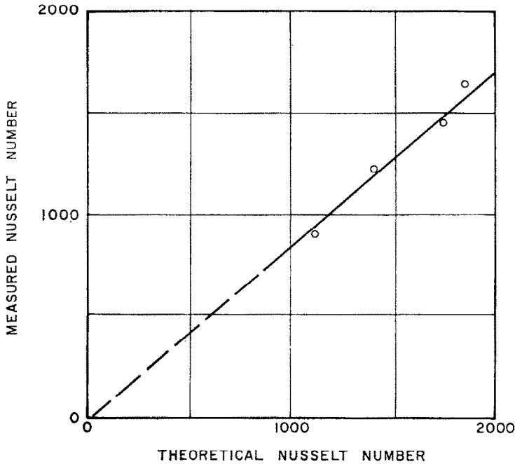
FIG. 6. Natural convection heat transfer across two 3 \times 3 in square openings spaced vertically 15 in apart on centers in a 2\frac{1}{4} -in thick partition. (The Nusselt numbers are based on a height of 3 in and a total area of 18 sq. in.)
