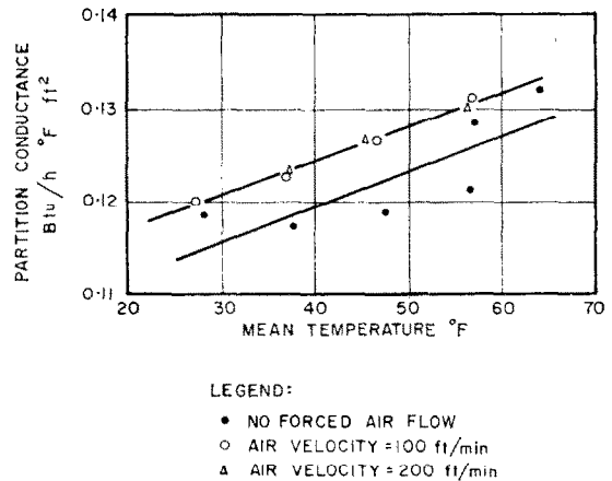
FIG. 3. Calibration of the test partition.
