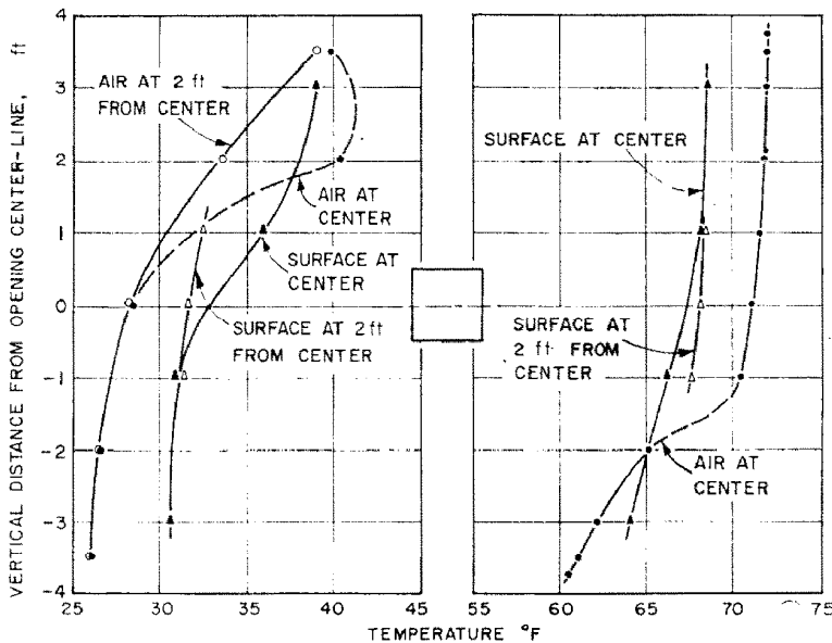
FIG. 4. Air and surface temperatures about a 12 × 12-in opening in a 2¼-in insulated partition.
