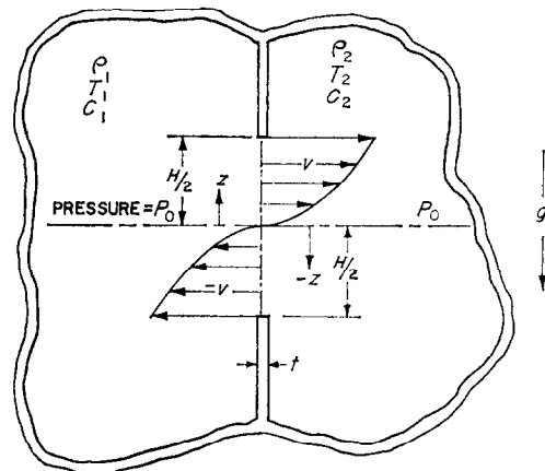
FIG. 1. Schematic representation of natural convection across an opening in a vertical partition.
