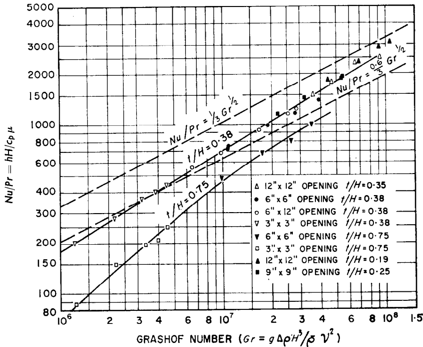
FIG. 5. Natural convection across rectangular openings in a vertical partition.
