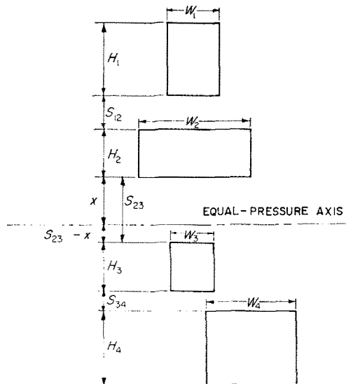
FIG. 8. Designation for multiple openings in a vertical wall.
