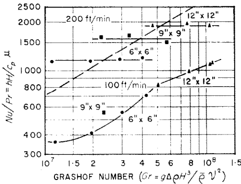
FIG. 7. Effect of a horizontal air flow parallel to the opening and partition. (The dashed curve is that for natural convection with t/H = 0.38 from Fig. 5.)
